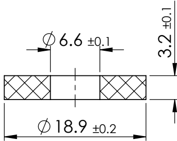
SECTION X-X
